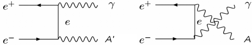
Figure 44. A' production via e^+e^- annihilation.
