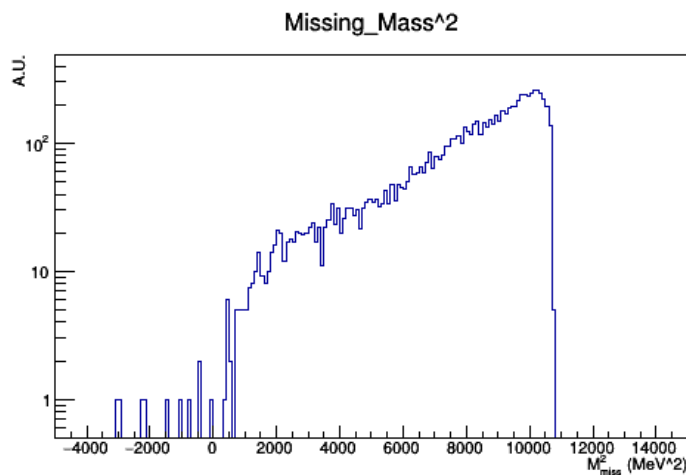
Figure 47. Calculated missing mass spectrum of 3 photons events.
