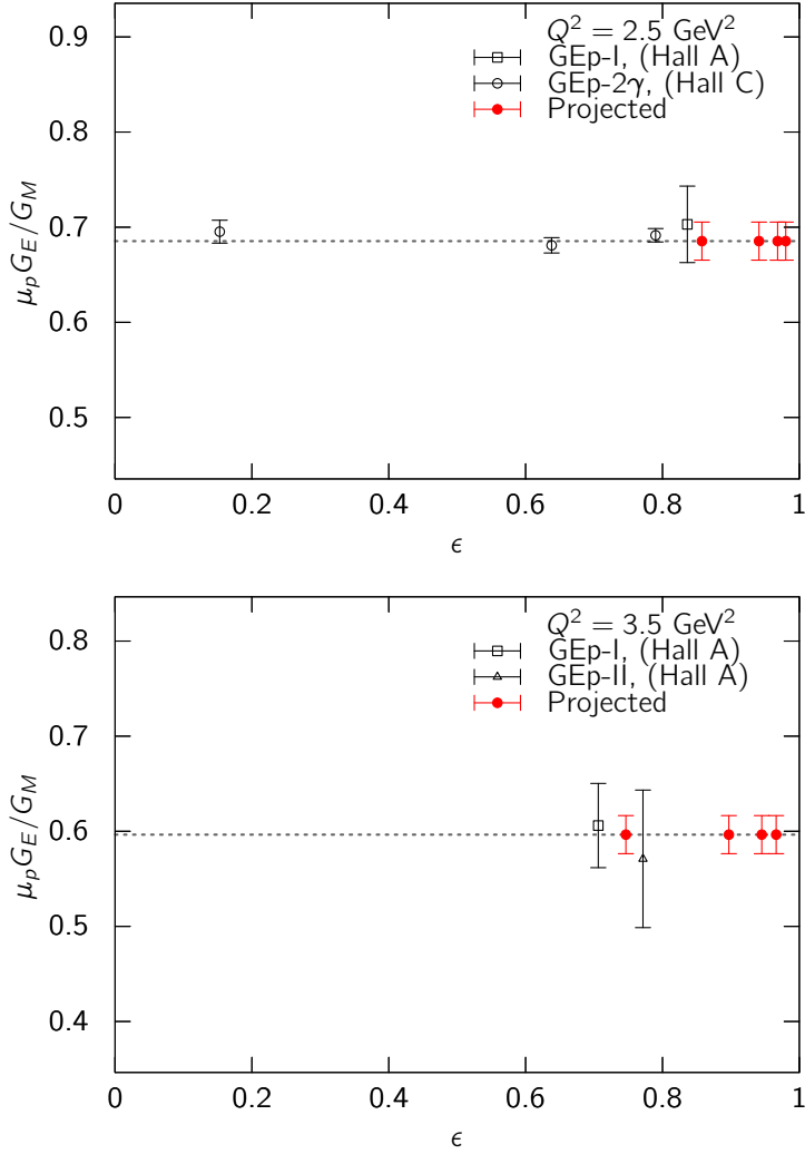
Figure 20. Previous polarization transfer data taken with electrons (black) is shown as a function of \epsilon in comparison to the kinematics of the projected positron measurement (red) with the target 2% statistical uncertainties.
