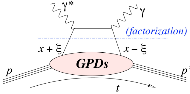
Figure 22. Leading order contributions to the production of high energy single photons from protons. The DVCS handbag diagram contains the information on the unknown GPDs.
