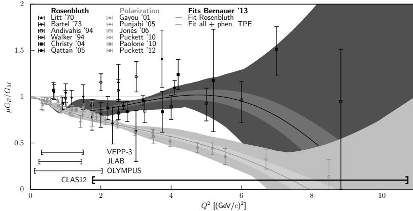
Figure 9. The proton form factor ratio \mu G_E/G_M , as determined via Rosenbluth-type (black points, from [Lit70, Bar73, And94, Wal94, Chr04, Qat05]) and polarization-type (gray points, from [Gay01, Pun05, Jon06, Puc10, Pao10, Puc12]) experiments. While the former indicate a ratio close to 1, the latter show a distinct linear fall-off. Curves are from a phenomenological fit [Ber14], to either the Rosenbluth-type world data set alone (dark curves) or to all data, then including a phenomenological two-photon-exchange model. We also indicate the coverage of earlier experiments as well as of the experiment described below.
