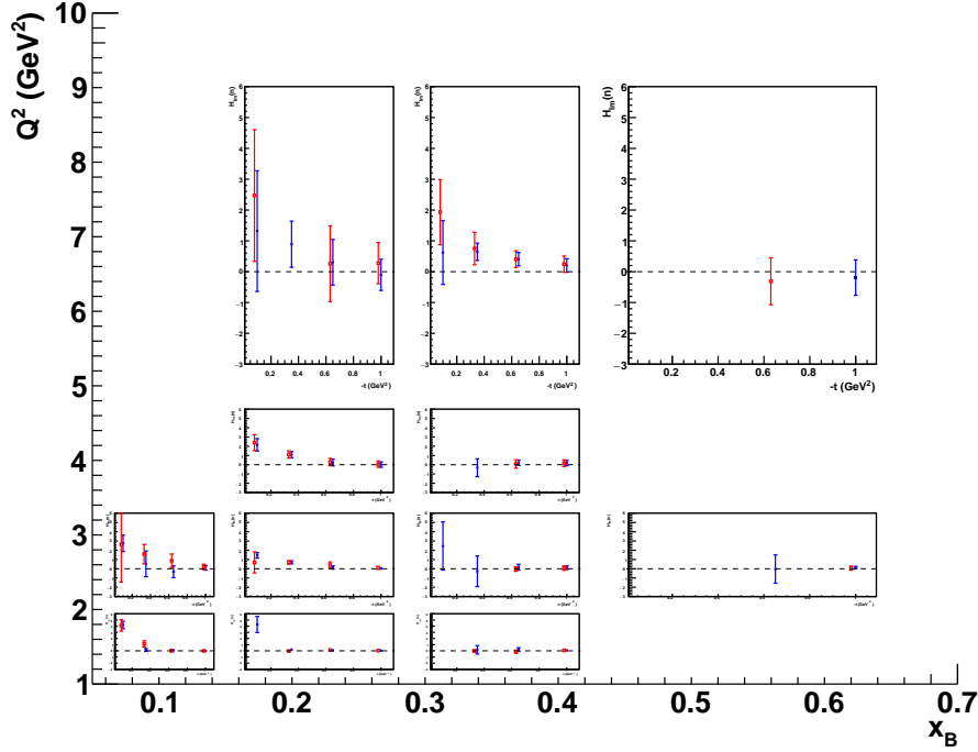
Figure 37. H_{Im}(n) as a function of -t , for all bins in Q^2 and x_B . The blue points are the results of the fits including the proposed BCA while the red ones include only already approved experiments.
