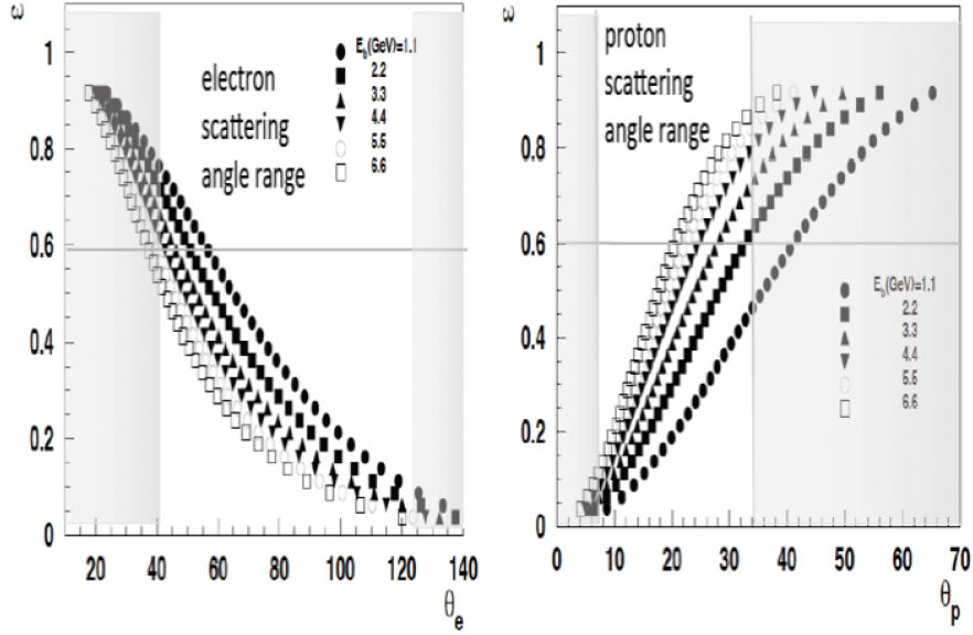
Figure 12. Polar angle and \varepsilon coverage for electron detection (left) and for proton detection (right).
