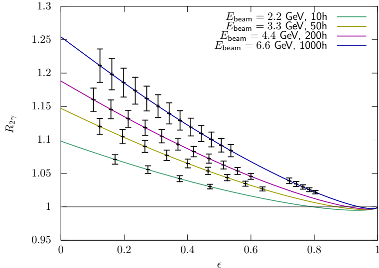
Figure 15. Predicted effect size and estimated errors for the proposed measurement program at CLAS12. We assume bins of constant \Delta Q^2=0.25 \text{ GeV}^2 .
