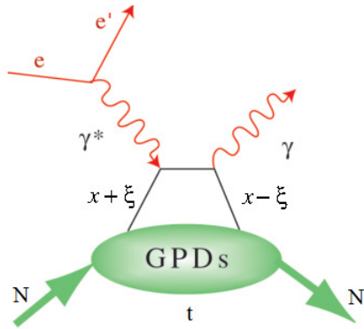
Figure 28. The handbag diagram for the DVCS process on the nucleon eN \rightarrow e'N'\gamma' ; here x+\xi and x-\xi are the longitudinal momentum fractions of the struck quark before and after scattering, respectively, and t = (N - N')^2 is the squared four-momentum transfer between the initial and final nucleons. \xi \simeq x_B/(2 - x_B) is proportional to the Bjorken scaling variable x_B = Q^2/2M\nu , where M is the nucleon mass and \nu is the energy transferred to the quark.
