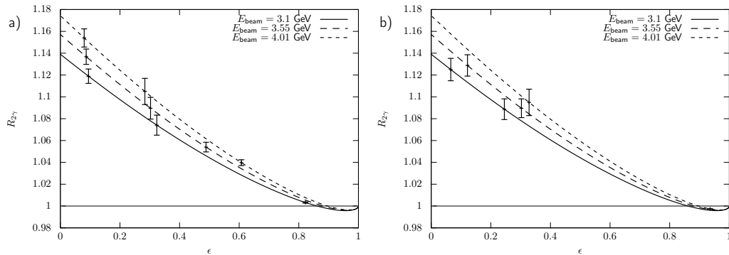
Figure 16. Predicted effect size and estimated errors for the proposed measurement program in Hall A (a) and Hall C (b).
