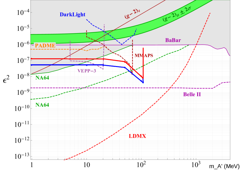
Figure 49. Projected exclusion limits in the A' invisible decay parameter space for a 180 days experiment with a 10 nA (red curve) and 100 nA (blue curve) 11 GeV positron beam at Jefferson Lab.
