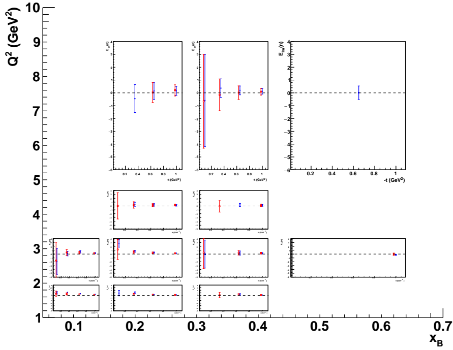
Figure 35. E_{Im}(n) as a function of -t , for all bins in Q^2 and x_B . The blue points are the results of the fits including the proposed BCA while the red ones include only already approved experiments.
