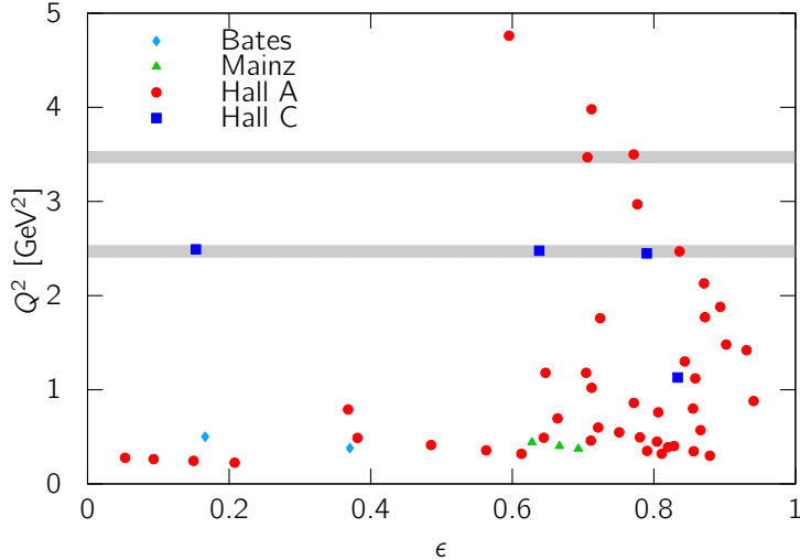
Figure 19. The kinematics of previous polarization transfer measurements with electron beams are shown. A measurement with positrons at either Q^2 = 2.5 \text{ GeV}^2 or 3.5 \text{ GeV}^2 would be able to compare with previous electron experiments.
