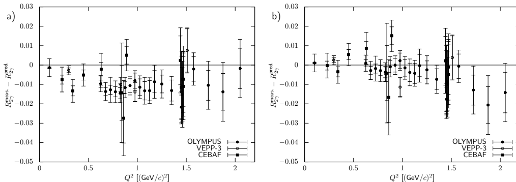
Figure 11. Difference of the data of the three recent TPE experiments [Rac15, Rim17, Hen17] to the calculation in [Blu17] (a) and the phenomenological prediction from [Ber14] (b).
