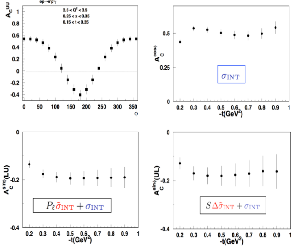
Figure 24. Electron-positron DVCS charge asymmetries: (top-left) azimuthal dependence of the charge asymmetry for positron and electron beam at 11 GeV beam; (top-right) moment in \cos(\phi) of the charge asymmetry versus momentum transfer t to the proton; (bottom-left) charge asymmetries for polarized electron and positron beams at fixed polarization (LU); (bottom right) charge asymmetry for longitudinally polarized protons at fixed polarization (UL). The error bars are estimated for a 1000 hours run with positron beam and luminosity \mathcal{L} = 2 \times 10^{34} \text{ cm}^{-2} \cdot \text{sec}^{-1} at a beam polarization P = 0.6 , and a 1000 hours electron beam run with luminosity \mathcal{L} = 10 \times 10^{34} \text{ cm}^{-2} \cdot \text{sec}^{-1} and beam polarization P = 0.8 . The error bars are statistical for a single bin in Q^2 , x , and t as shown in the top-left panel. Other bins are measured simultaneously.
