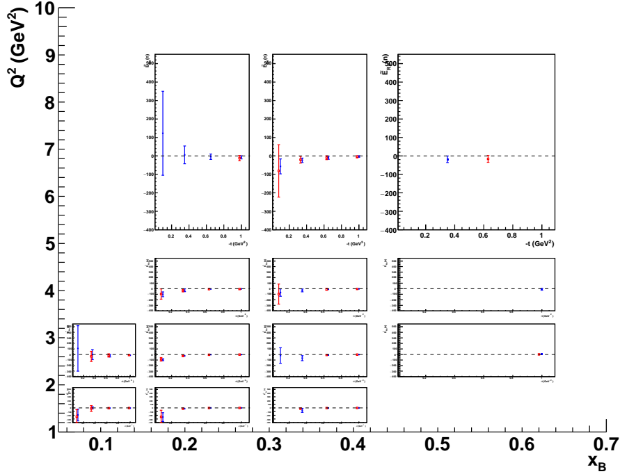
Figure 34. \widetilde{E}_{Re}(n) as a function of -t , for all bins in Q^2 and x_B . The blue points are the results of the fits including the proposed BCA while the red ones include only approved experiments.
