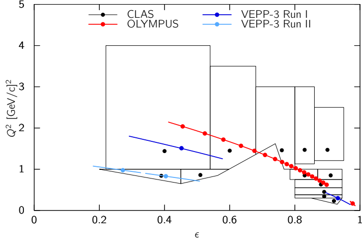
Figure 10. Kinematics covered by the three recent experiments to measure the two-photon exchange contribution to the elastic ep cross section.
