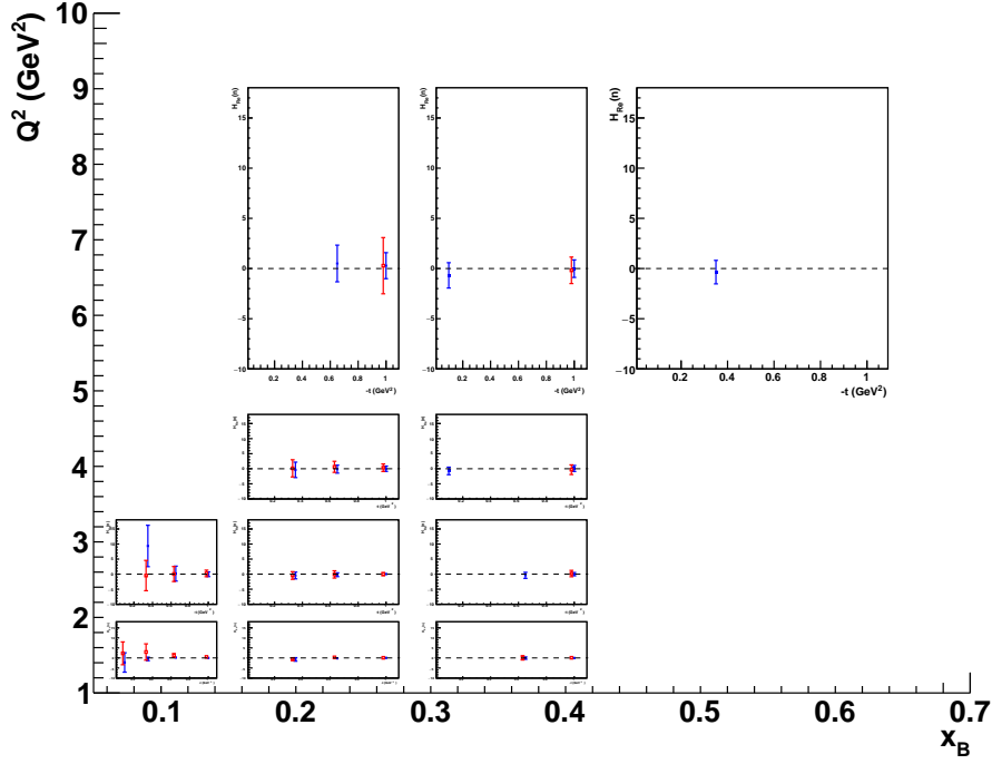
Figure 33. H_{Re}(n) as a function of -t , for all bins in Q^2 and x_B . The blue points are the results of the fits including the proposed BCA while the red ones include only already approved experiments.
