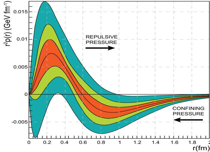
Figure 26. The radial pressure distribution in the proton. The graph shows the pressure distribution r^2 p(r) resulting from the interactions of the quarks in the proton versus the radial distance from the center in femtometer. The black central line corresponds to the pressure extracted from the D -term parameters fitted to the published data at 6 GeV [Jo15]. The corresponding estimated uncertainties are displayed as the shaded area shown in light green. Uncertainties represent 1 standard deviation.
