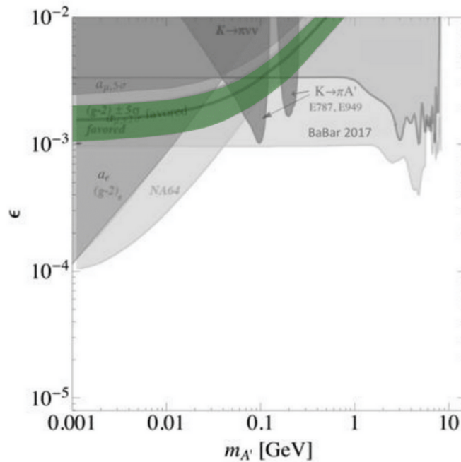
Figure 43. Current exclusion limits for A' invisible decay.
