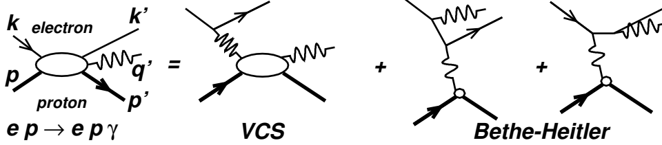
Figure 38. Lowest order QED amplitude for the ep \rightarrow ep\gamma reaction. The momentum four-vectors of all external particles are labeled at left. The net four-momentum transfer to the proton is \Delta_\mu = (q - q')_\mu = (p' - p)_\mu . In the virtual Compton scattering (VCS) amplitude, the (spacelike) virtuality of the incident photon is Q^2 = -q^2 = -(k - k')^2 . In the Bethe-Heitler (BH) amplitude, the virtuality of the incident photon is -\Delta^2 = -t . Standard (e, e') invariants are s_e = (k + p)^2 , x_B = Q^2/(2q \cdot p) and W^2 = (q + p)^2 .
