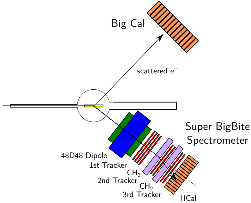
Figure 18. A schematic of the proposed PT measurement.
