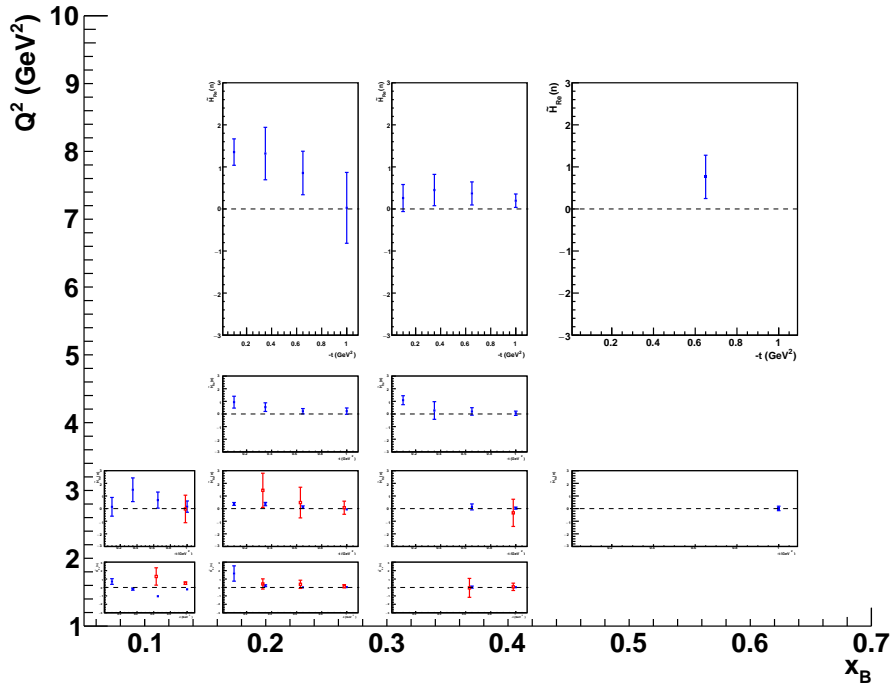
Figure 32. \widetilde{H}_{Re}(n) as a function of -t , for all bins in Q^2 and x_B . The blue points are the results of the fits including the proposed BCA while the red ones include only already approved experiments.
