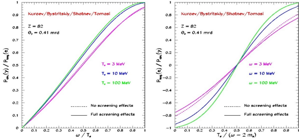
Figure 3. (left) The circular polarization of the photons produced by longitudinally polarized electrons at a fixed production angle of 0.41 mrad for several electron beam energies and for the extreme cases of full- or no-screening as a function of the ratio of the photon energy to the electron energy [Kur10, Vou17]. (right) The electron/positron longitudinal polarization resulting from the pair production by circularly polarized photons for the extreme cases of full- or no- screening for several photon beam energies as a function of the ratio of the positron energy to the photon beam energy less the sum of the electron and positron masses [Kur10, Vou17].
