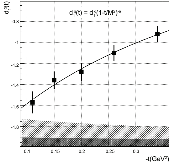
Figure 25. Example of a fit to d_1(t) . The error bars are from the fit to the cross sections at fixed value of -t . The single-shaded area at the bottom corresponds to the uncertainties from the extension of the fit into regions without data and is reflected in the green shaded area in Fig. 26. The double-shaded area corresponds with the projected uncertainties from future experiment [Elo16], as shown in Fig. 26 with the red shaded area. Uncertainties represent 1 standard gaussian deviation.
