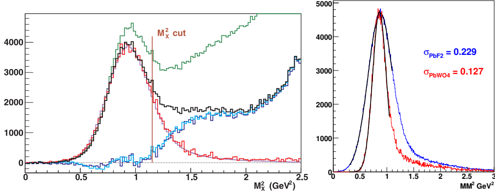
Figure 40. (left) Missing mass squared in E00-110 for H(e, e'\gamma)X events (green curve) at Q^2 = 2.3 \text{ GeV}^2 and -t \in [0.12, 0.4] \text{ GeV}^2 , integrated over the azimuthal angle of the photon \phi_{\gamma\gamma} . The black curve shows the data once the H(e, e'\gamma)\gamma X' events have been subtracted. The other curves are described in the text. (right) Projected missing mass resolution for a similar kinematic setting ( E_b = 6.6 \text{ GeV} , Q^2 = 3 \text{ GeV}^2 , x_B = 0.36 ). By using \text{PbWO}_4 instead of \text{PbF}_2 , the missing mass resolution will be considerably improved. Values are given in Tab. 6 and are to be compared to the value \sigma(M_X^2) = 0.2 \text{ GeV}^2 obtained in previous experiments in Hall A.
