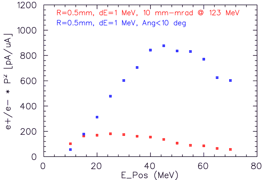
Figure 8. The Figure of Merit ( P_z^2 I ) for the positron beam produced by a 123 MeV 85% longitudinally polarized electron beam as a function of the positron energy [15]. As is the case for the curves in Fig. 6, the red data points correspond to the selection of produced positrons within an energy spread of 1 MeV and a normalized emittance of 2400 mm mr, while the blue data points correspond to selection with the same energy spread but within a constant angular acceptance of 10 deg.
