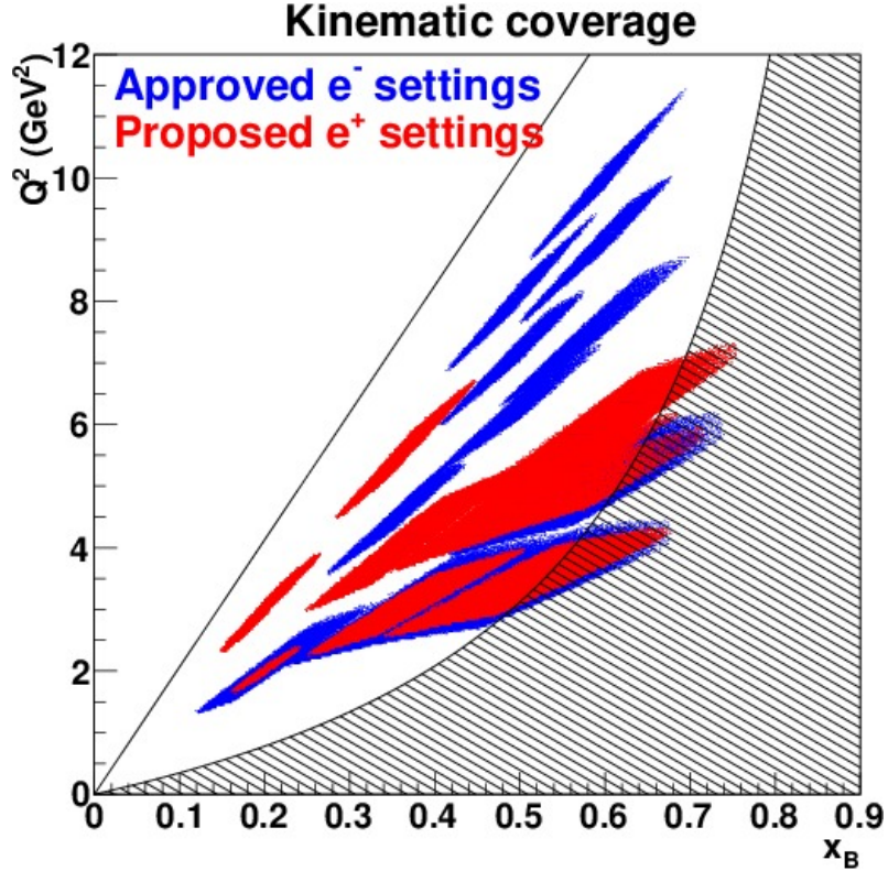
Figure 41. Display of the different kinematic settings proposed. Blue corresponds to the settings already approved in Hall A and Hall C using an electron beam. Red shows the proposed kinematics with positrons. Shaded areas show the resonance region W < 2 \text{ GeV} and the line Q^2 = (2M_p E_b)x_B limits the physical region for a maximum beam energy E_b=11 \text{ GeV} .
