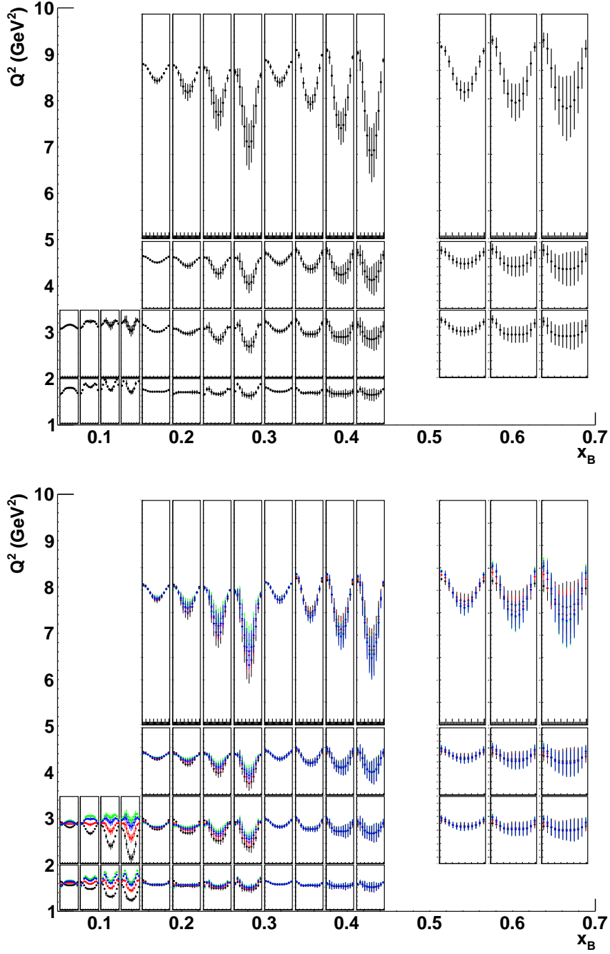
Figure 30. Projected BCA data for the D(e, en\gamma)p reaction as predicted by the VGG model for (J_u, J_d) = (0.3, 0.1) (top) and alternative combinations (bottom). The bottom plot compares (J_u, J_d) : (0.3, 0.1) (black), (0.2, 0.0) (red), (0.1, -0.1) (green), and (0.3, -0.1) (blue). The vertical axis scale ranges from -0.3 to 0.1 for the top plot and from -0.3 to 0.2 for the bottom plot. The error bars reflect the expected statistical uncertainties for 80 days of beam time at a luminosity of 10^{35} \text{ cm}^{-2} \cdot \text{s}^{-1} per nucleon.
