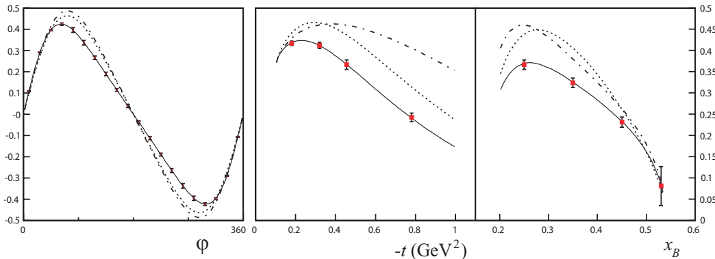
Figure 23. The beam spin asymmetry showing the DVCS-BH interference for 11 GeV beam energy [Sab11]: (left panel) x = 0.2 , Q^2 = 3.3 \text{ GeV}^2 , -t = 0.45 \text{ GeV}^2 ; (middle and right panels) \phi = 90^\circ , other parameters same as in left panel. Many other bins will be measured simultaneously. The curves represent various parameterizations within the VGG model [Van99]. Projected uncertainties are statistical.
