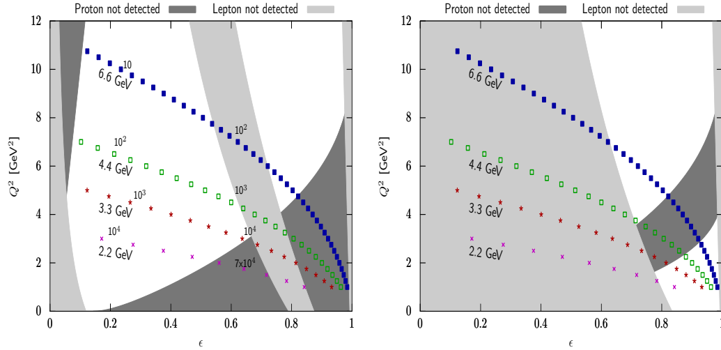
Figure 13. Expected elastic event rates per hour for energies 2.2, 3.3, 4.4, 6.6 GeV in the \varepsilon - Q^2 plane. Shaded areas are excluded by the detector acceptance. Left: proposed experiment; Right: standard setup
