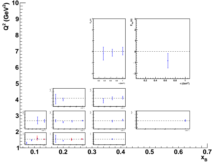
Figure 31. E_{Re}(n) as a function of -t , for all bins in Q^2 and x_B . The blue points are the results of the fits including the proposed BCA while the red ones include only already approved experiments.
