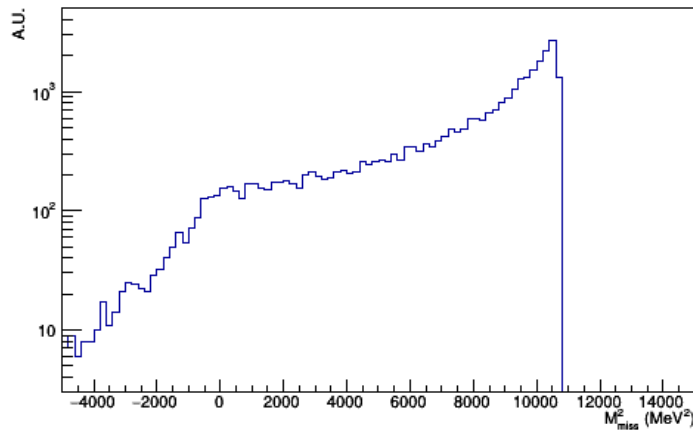
Figure 46. Calculated missing mass spectrum of bremsstrahlung events.
