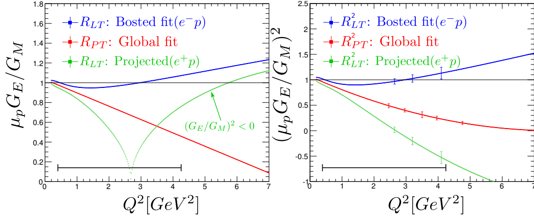
Figure 22. Parameterizations of R = \mu_p G_E / G_M (left) and R^2 (right) from LT and polarization data, along with the results expected for positrons assuming that TPE corrections fully explain the LT-Polarization discrepancy. The right figure indicates the Q^2 range that could be covered under the assumptions provided in the text, and the point for the electron and positron R_{LT}^2 results indicate the uncertainties from the previous Hall A Super-Rosenbluth extraction [Qat05].
