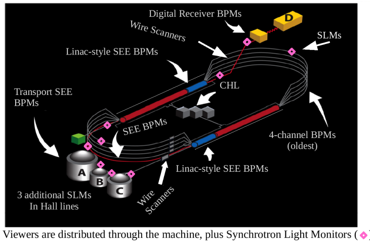
Figure 13. Beam diagnostic systems and their distribution in the CEBAF accelerator.
