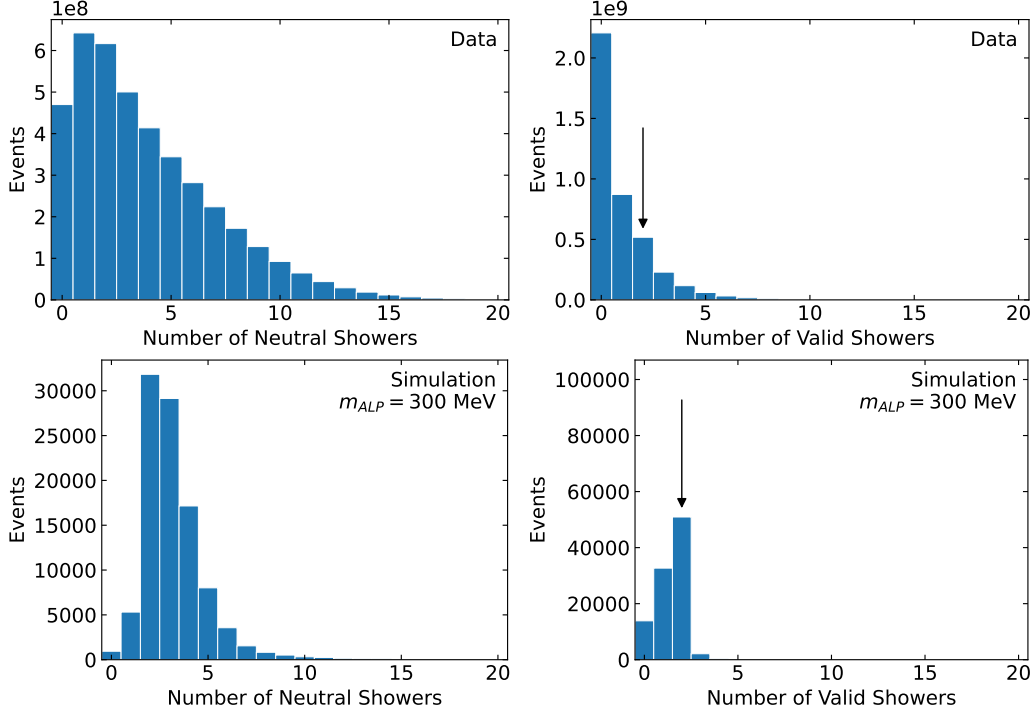
Figure 7: Top left: The total number of neutral showers per event in a subset of data. Top right: The number of neutral showers satisfying the listed requirements per event in a subset of data. Events required exactly two such showers, with extra showers initially ignored. Bottom: Same as top figures in simulated signal with m_{\chi} = 300 MeV. Shower validity conditions may be seen to be generally applicable for signal events.
