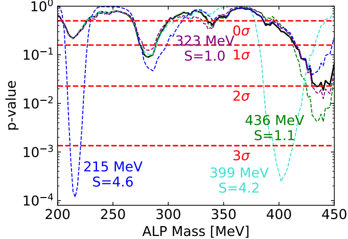
Figure 28: Local p-value for signal discovery over the examined mass range. The black curve shows the p-value for the existing dataset, while the colored curves show the p-value after random signal injection.
