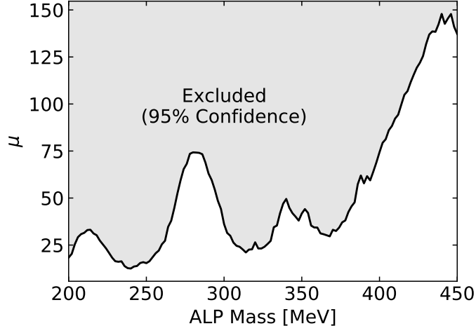
Figure 31: 95% exclusion range on \mu as a function of m_a .
