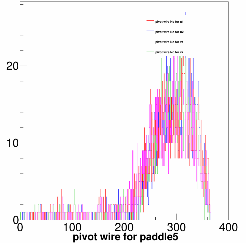
Tritium cosmic run
