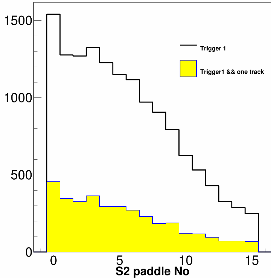
GMP cosmic run
