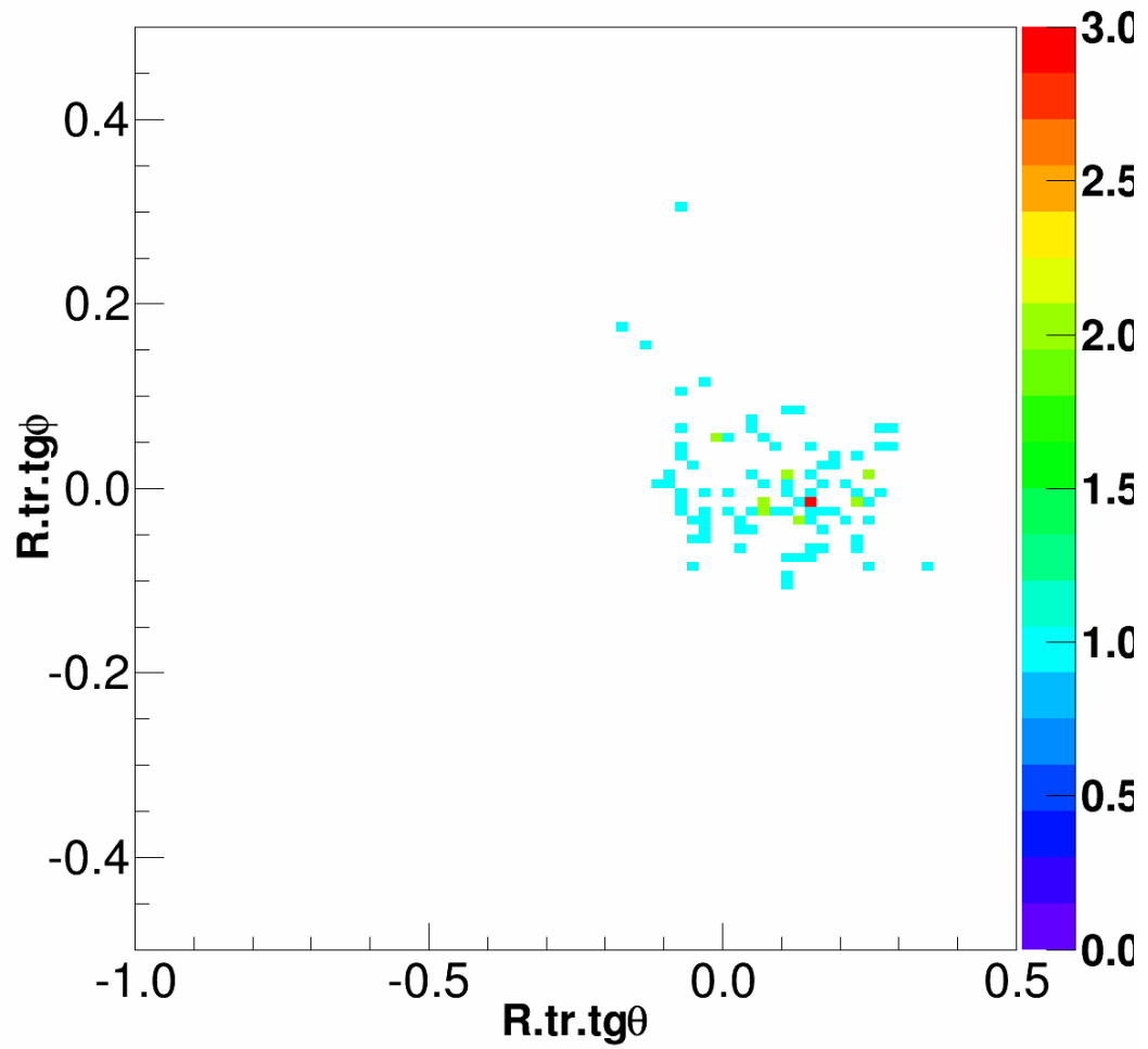
GMP cosmic run
