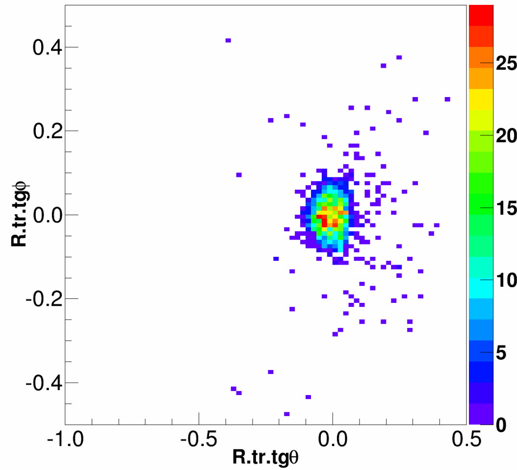
Tritium cosmic run
