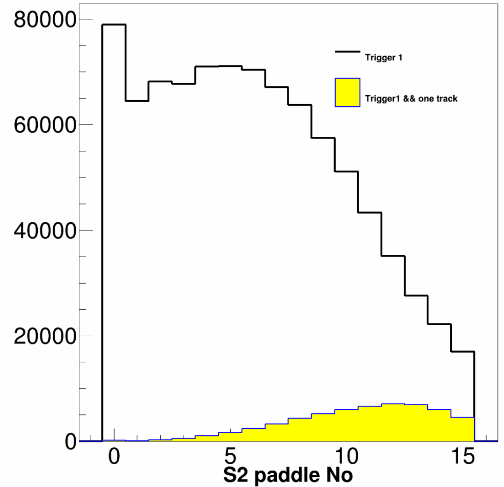
Tritium cosmic run
