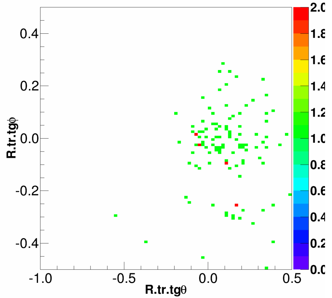
Tritium cosmic run
