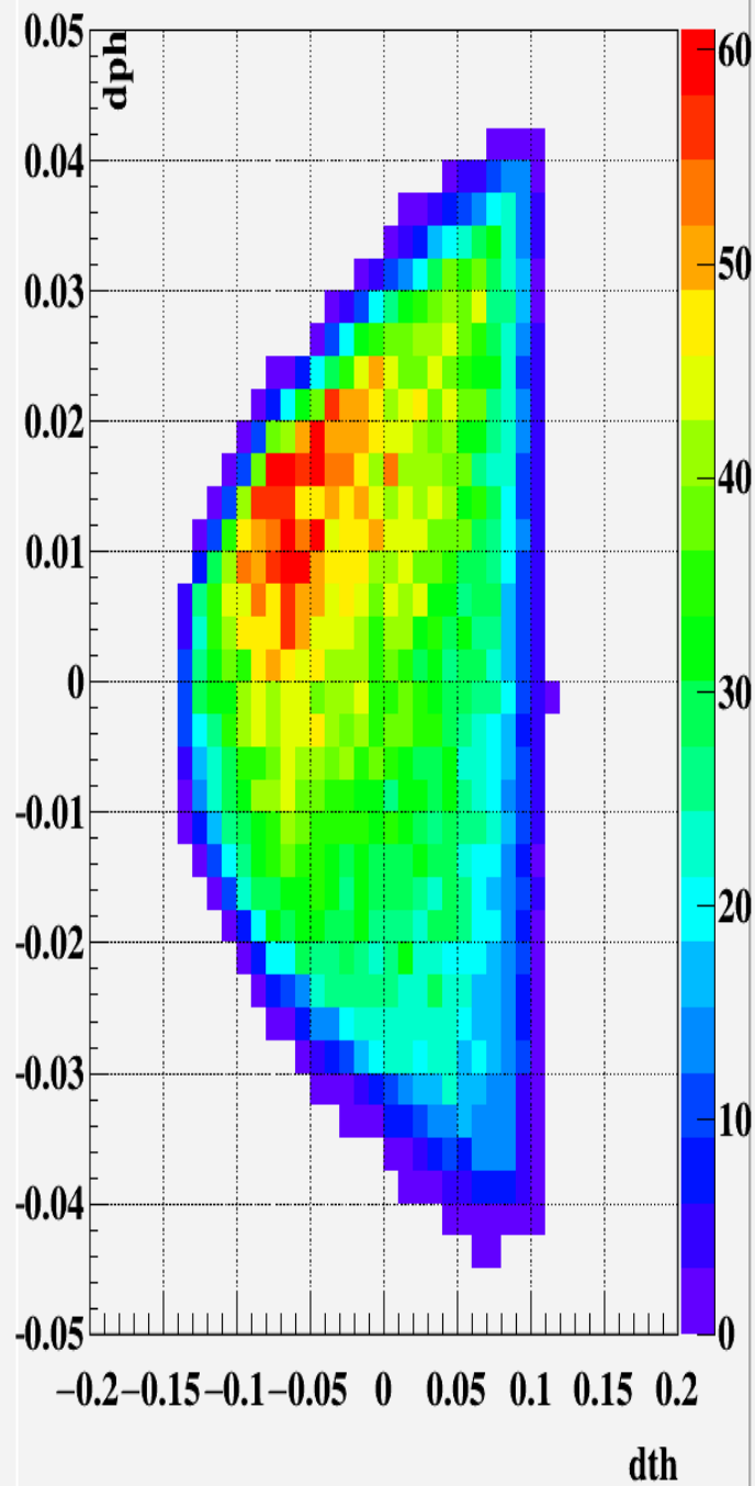
yp(ph):xp(th) run1207
