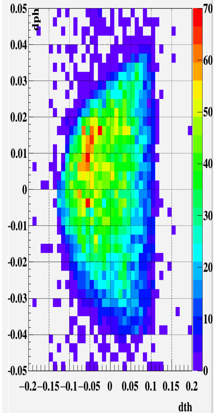
yp(ph):xp(th) run1207
